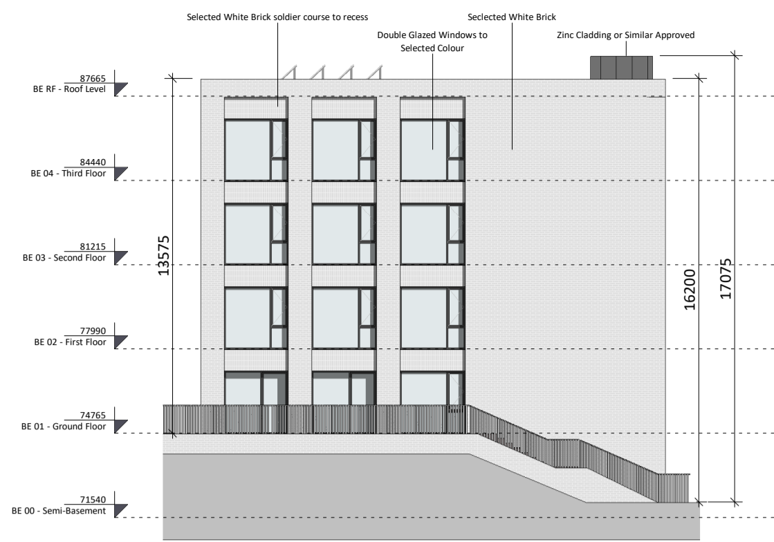
1 Block E East Elevation 1 : 200
