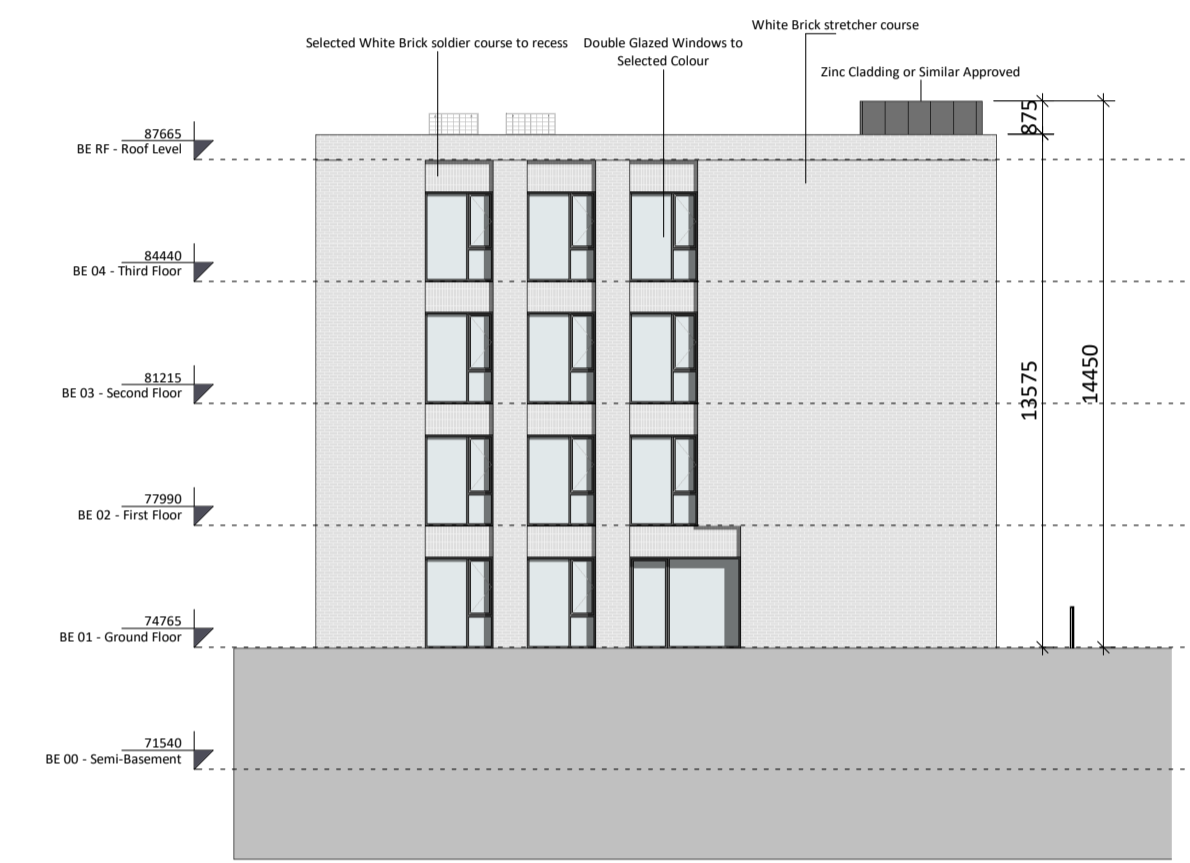
3 Block E South Elevation 1 : 200
